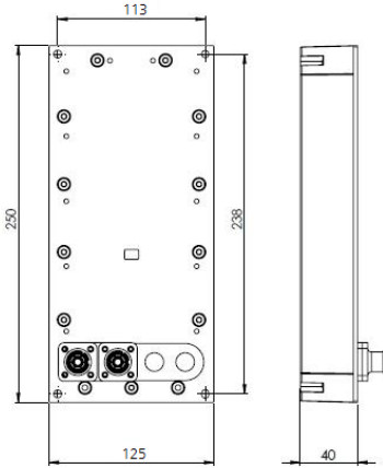
Bird-80A
